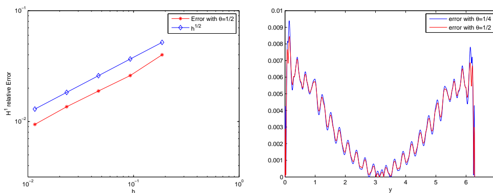
Fig. 7. Relative H^1 error versus the mesh size, in logarithmic scales, for \theta = \frac{1}{2} (left), and error on the interface for \theta = \frac{1}{4} and for \theta = \frac{1}{2} (right)
