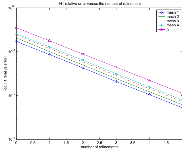
Fig. 5. Relative H^1 error versus the number of refinements for the initial meshes : mesh 1, (diamond line), mesh 2 (solid line), mesh 3 (dashed line), and mesh 4 (star line). The triangle line is the mesh size h versus the number of refinements, in logarithmic scale
