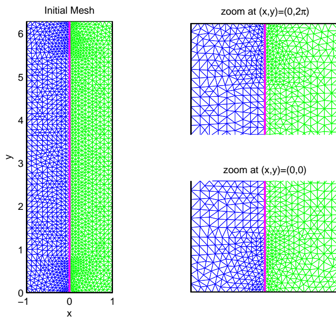
Fig. 6. Initial non-conforming meshes: global meshes (left) with a zoom at corners (right)
