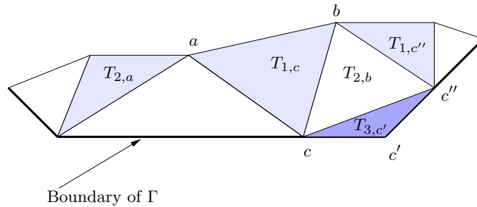
Fig. 1. Two different situations of 2D triangulation of the interface \Gamma , next to its boundary (near cross points): in light grey (triangle labeled 1) a vertex c is connected to two vertices in the interior of \Gamma , in dark grey (triangle labeled 3) a vertex c' is connected to two vertices on the boundary of \Gamma
