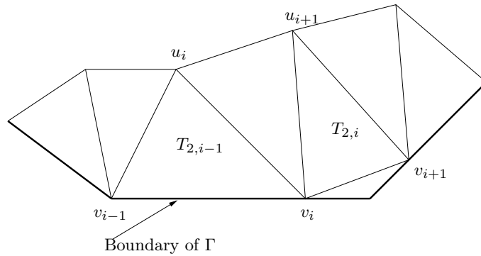
Fig. 2. Notations for the triangles having two vertices on the boundary of \Gamma (triangle of type 2)
