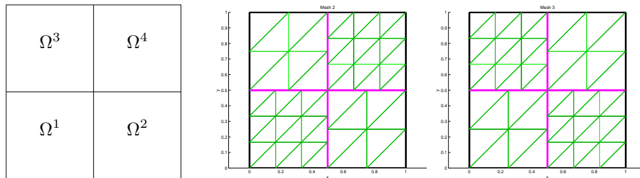
Fig. 4. Domain decomposition (on the left), and non-conforming meshes: mesh 2 (on the middle), and mesh 3 (on the right)
