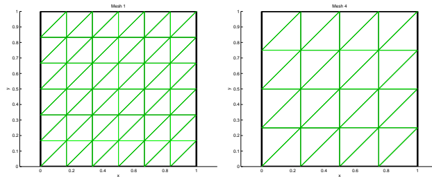
Fig. 3. Uniform conforming meshes : mesh 1 (on the left), and mesh 4 (on the right)
