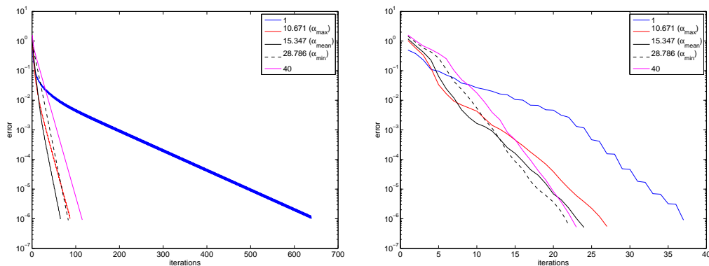
Fig. 9. Relative H^1 error between the discrete Schwarz (left part) and Gmres (right part) converged solution and the iterate solution, for different values of the Robin parameter \alpha
