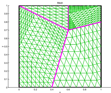
Fig. 8. Domain decomposition in 4 subdomains with non-conforming grids
