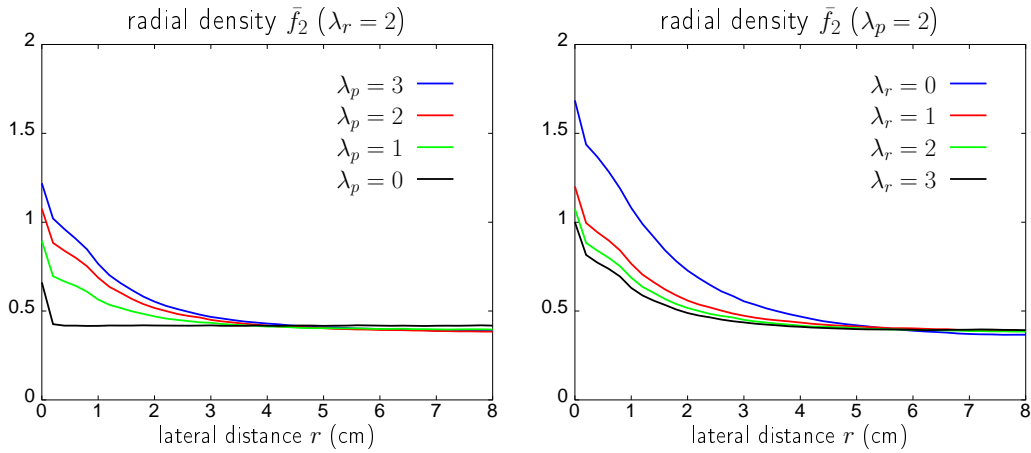
Figure 11: (Left) \bar{f}_2(r) as a function of r for different values of the trail recruitment frequency \lambda_p and a fixed value of the random jump frequency equal to \lambda_r = 2 \text{ s}^{-1} . (Right) \bar{f}_2(r) as a function of r for different values of the random jump frequency \lambda_r and a fixed value of the trail recruitment frequency equal to \lambda_p = 2 \text{ s}^{-1} .
