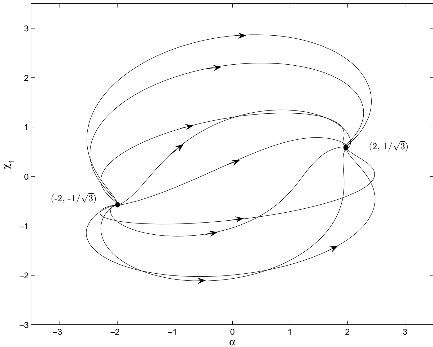
\alpha and \chi_1 phase space
