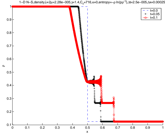
(a) Density
