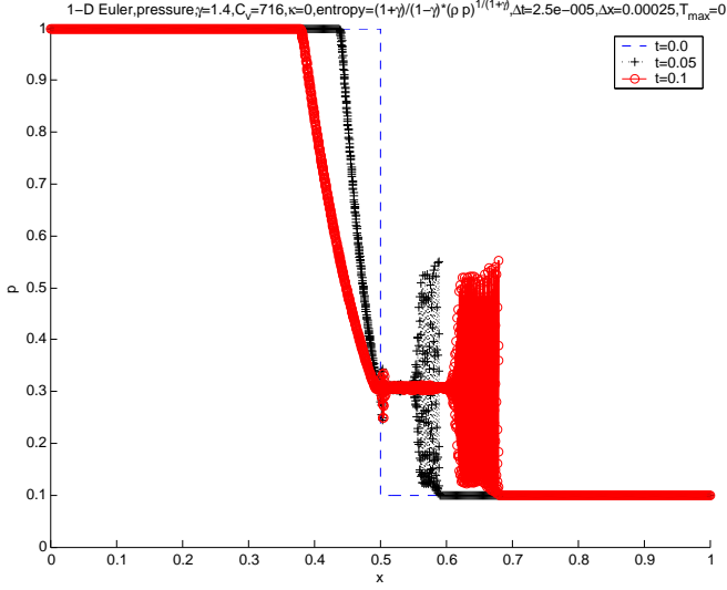
(c) Pressure
