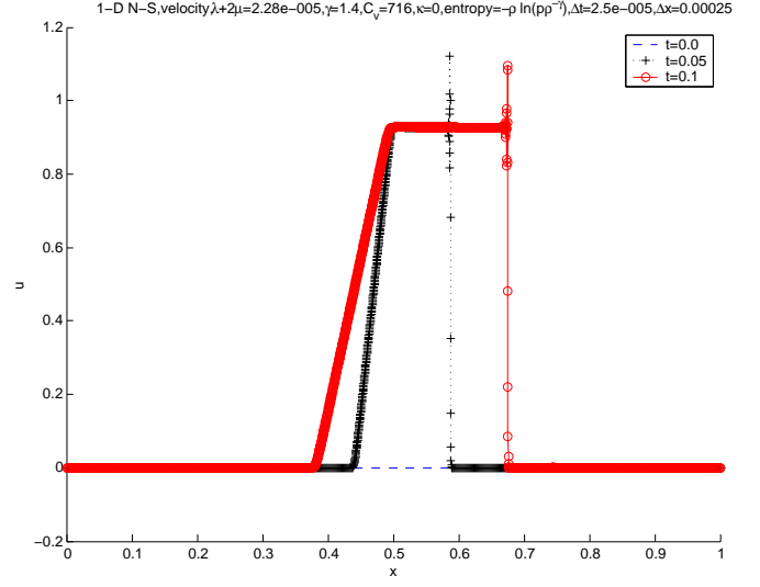
(b) Velocity
