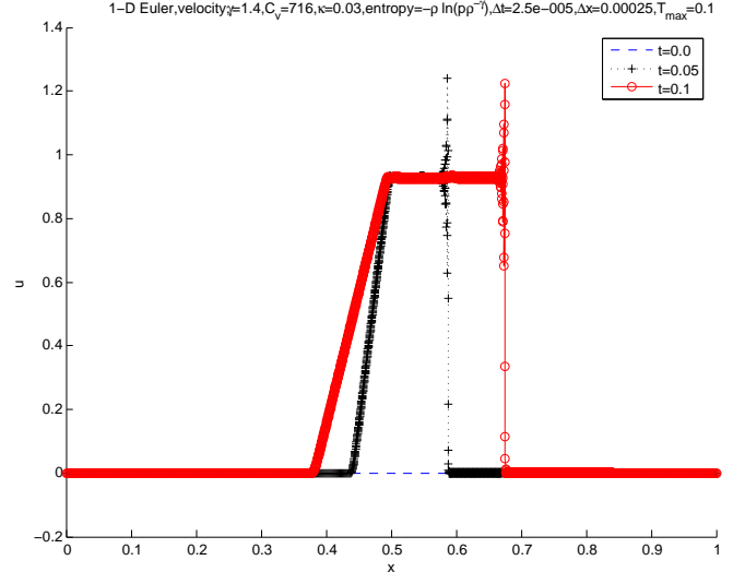
(b) Velocity
