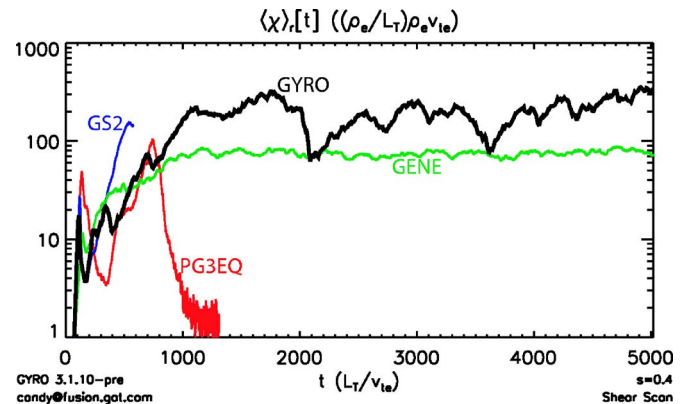
FIG. 14. (Color online) \chi_e \equiv -Q_e / n_0 \nabla T_0 at s=0.4 from GYRO (black curve), GS2 (blue curve), GENE (green curve), and PG3EQ (red curve). The late-time ( t > 750 L_T / v_{te} ) drop in \chi_e from PG3EQ is due to the accumulation of discrete particle noise (Ref. 21).
