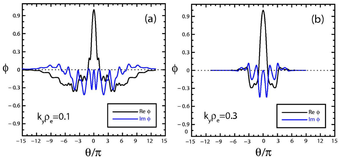
FIG. 2. (Color online) The linear eigenfunctions from GYRO are plotted vs \theta for \theta_0=0 and (a) k_y \rho_e=0.1 and (b) k_y \rho_e=0.3 . In both cases the real part is shown in black and the imaginary part is shown in blue. The eigenfunctions are normalized to equal 1.0 at \theta=0 .
