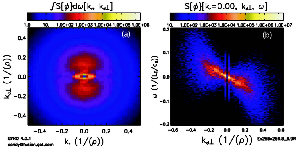
FIG. 11. (Color online) Spectral density of electrostatic potential fluctuations at the s=0.1 benchmark point (a) vs (k_r, k_\perp) and (b) vs (k_\perp, \omega) .
