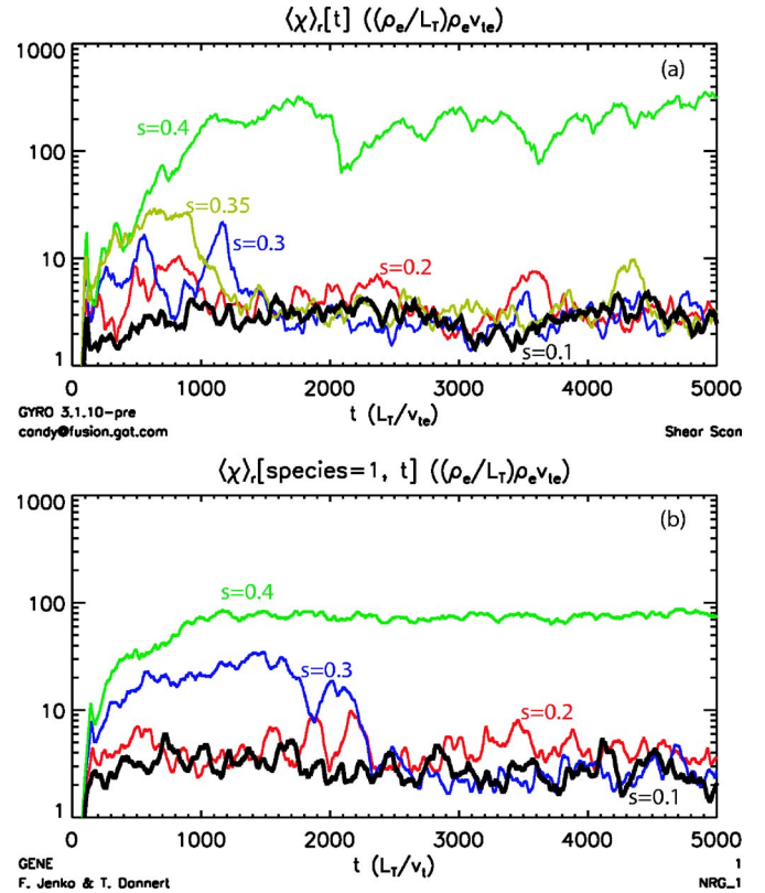
FIG. 13. (Color online) \chi_e \equiv -Q_e / n_0 \nabla T_0 , from a sequence of simulations with flux-tube cross section of L_x = 100 \rho_e by L_y = 64 \rho_e using (a) GYRO in which the magnetic shear is varied through s=0.1 (black curve), s=0.2 (red curve), s=0.3 (blue curve), s=0.35 (olive curve), and s=0.4 (green curve); and (b) GENE in which the magnetic shear is varied through s=0.1 (black curve), s=0.2 (red curve), s=0.3 (blue curve), and s=0.4 (green curve).
