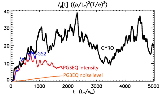
FIG. 9. (Color online) The fluctuation intensity, \langle \delta\phi^2 \rangle , averaged over the outboard midplane from GYRO (black curve), GS2 (blue curve), and PG3EQ (red curve). The contribution of discrete particle noise to the PG3EQ fluctuation intensity is shown by the orange curve.
