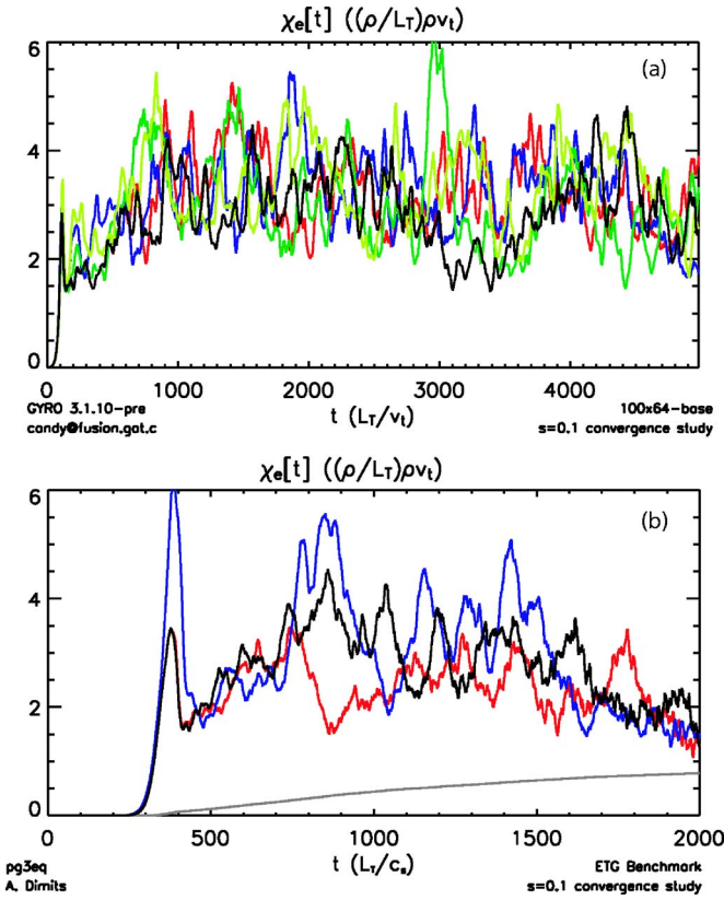
FIG. 3. (Color online) (a) Convergence study at the benchmark point from the GYRO code and (b) from the PG3EQ code. The black curves are the reference simulation. The time step is reduced by 1/2 for the red curve. The velocity space resolution is increased in the blue curves (from 128 to 288 velocity classes for GYRO; and from 16 to 32 particles/cell in PG3EQ). The green curve in (a) shows the effect of decreasing the radial grid spacing from dr \approx 2\rho_e to dr \approx 1.5\rho_e in GYRO, while the chartreuse curve shows the effect of increasing the poloidal resolution. The gray curve in (b) shows the contribution of the discrete particle noise to the total heat transport in the PG3EQ simulation (Ref. 21).
