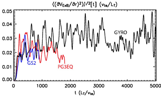
FIG. 12. (Color online) The rms flow shear is displayed vs time from GYRO (black curve), PG3EQ (red curve), and GS2 (blue curve).
