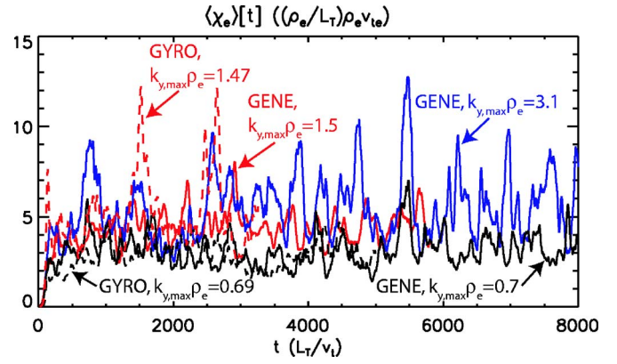
FIG. 4. (Color online) Convergence at the benchmark point in perpendicular grid resolution is investigated by comparing GENE simulations in an L_x=100\rho_e by L_y=62.82\rho_e flux tube with eight binormal modes such that k_{y,\max}\rho_e=0.7 (black curve), 16 k_y modes such that k_{y,\max}\rho_e=1.5 (red curve), and 32 k_y modes such that k_{y,\max}\rho_e=3.1 (blue curve). Gyro simulations with 8 k_y modes such that k_{y,\max}\rho_e=0.69 (dashed black curve) and 16 k_y modes such that k_{y,\max}\rho_e=1.47 (dashed red curve) are shown for comparison.
