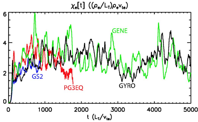
FIG. 8. (Color online) \chi_e \equiv -Q_e/n_0 \nabla T_0 , from GYRO (black curve), GS2 (blue curve), GENE (green curve), and PG3EQ (red curve) are plotted vs time.
