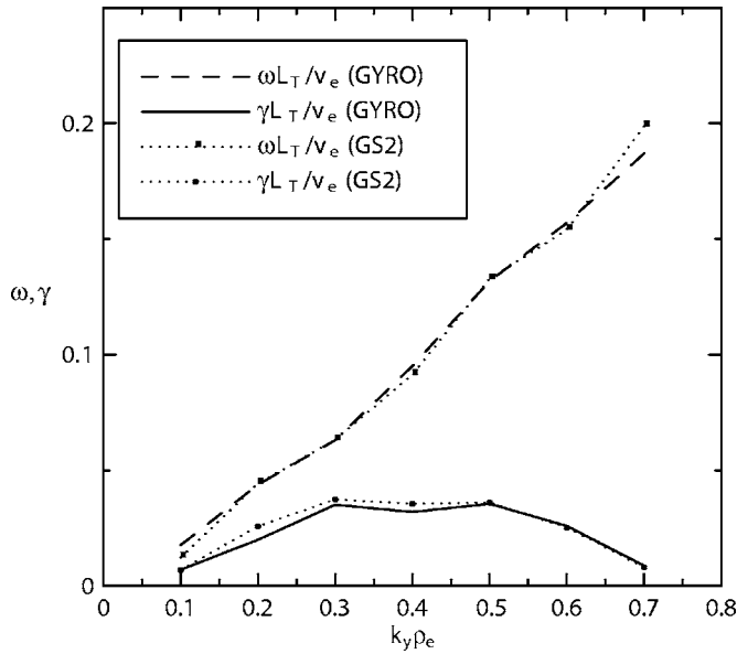
FIG. 1. Linear dispersion relation of ETG modes at the benchmark operating point vs k_y \rho_e as computed by GYRO and GS2 for linear eigenmodes with ballooning mode angle \theta_0=0 .
