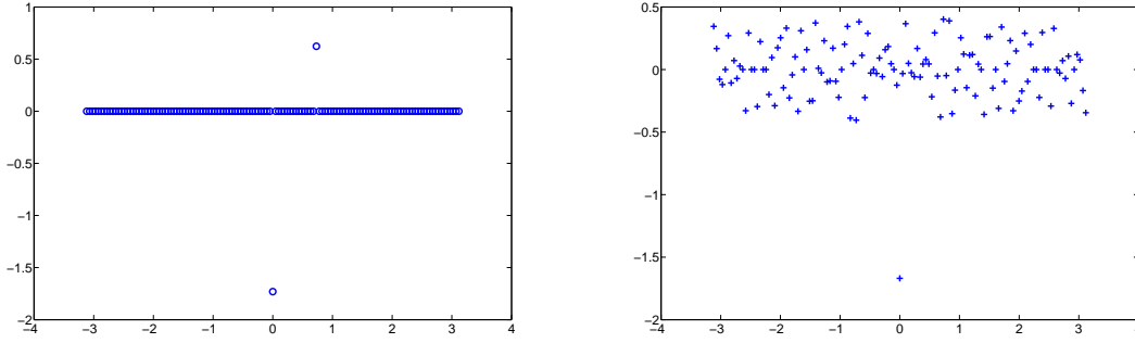
FIGURE 3.2. Demonstration of the sIFT edge detection method for recovering from noisy f_a(x) . Left: the results of the sIFT method. Right: the results of minmod detector (3.3).
