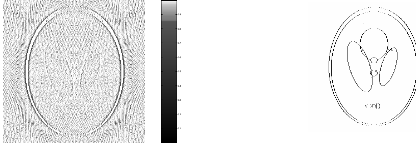
FIGURE 4.1. The recovered phantom image from incomplete spectral data. Left: the result by the standard back projection. Right: the recovered edges of Shepp-logan phantom graph by our compressed sensing edge detection method.
