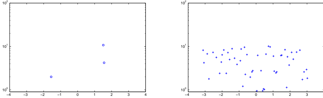
FIGURE 3.3. Demonstration of the sIFT edge detection method for recovering from noisy f_b(x) . Left: the results of the sIFT method. Right: the results of minmod method (3.3), where the true edges are concealed in the noisy data.
