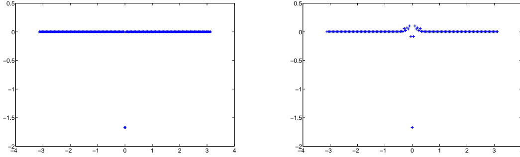
FIGURE 3.1. The recovery of [f_a](x) from its first N = 128 Fourier modes. The results of the sIFT edge detection method (on the left), and the results of \text{minmod} (3.3) on the right. Both experiments use \sigma(\theta) = 3\theta^3 corresponding to the unit mass concentration factor \hat{\eta}_3(\theta) = 3\theta^2 .
