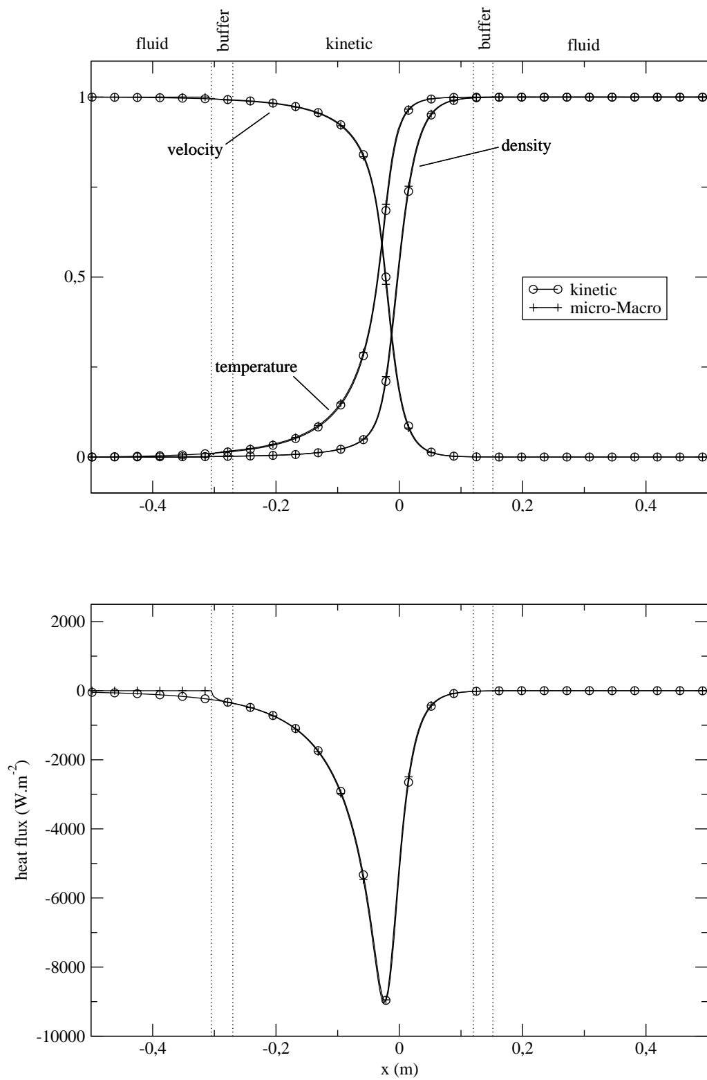
Figure 10: Density, velocity and temperature (top) and heat flux (bottom) for the stationary normal shock wave. Comparison of the full kinetic BGK equation to the micro-Macro model with a kinetic zone defined by a local Knudsen number greater than 10^{-3} .
