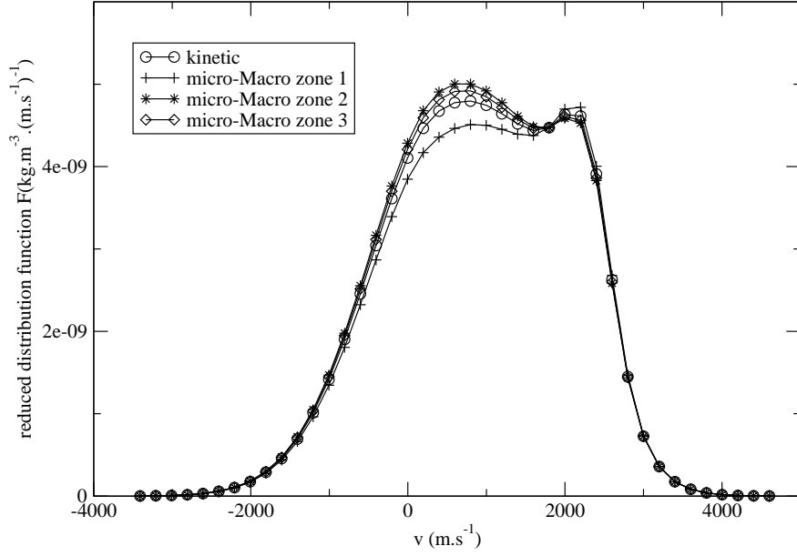
Figure 14: Stationary normal shock wave problem: reduced distribution function F(x, v) at x = 0 m (in the shock) for BGK and micro-Macro model used with three different kinetic zones (1: Kn > 10^{-2} , 2: Kn > 10^{-2} , 3: Kn > 10^{-2} ).
