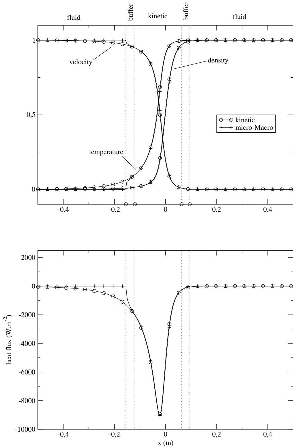
Figure 9: Density, velocity and temperature (top) and heat flux (bottom) for the stationary normal shock wave. Comparison of the full kinetic BGK equation to the micro-Macro model with a kinetic zone defined by a local Knudsen number greater than 10^{-2} .
